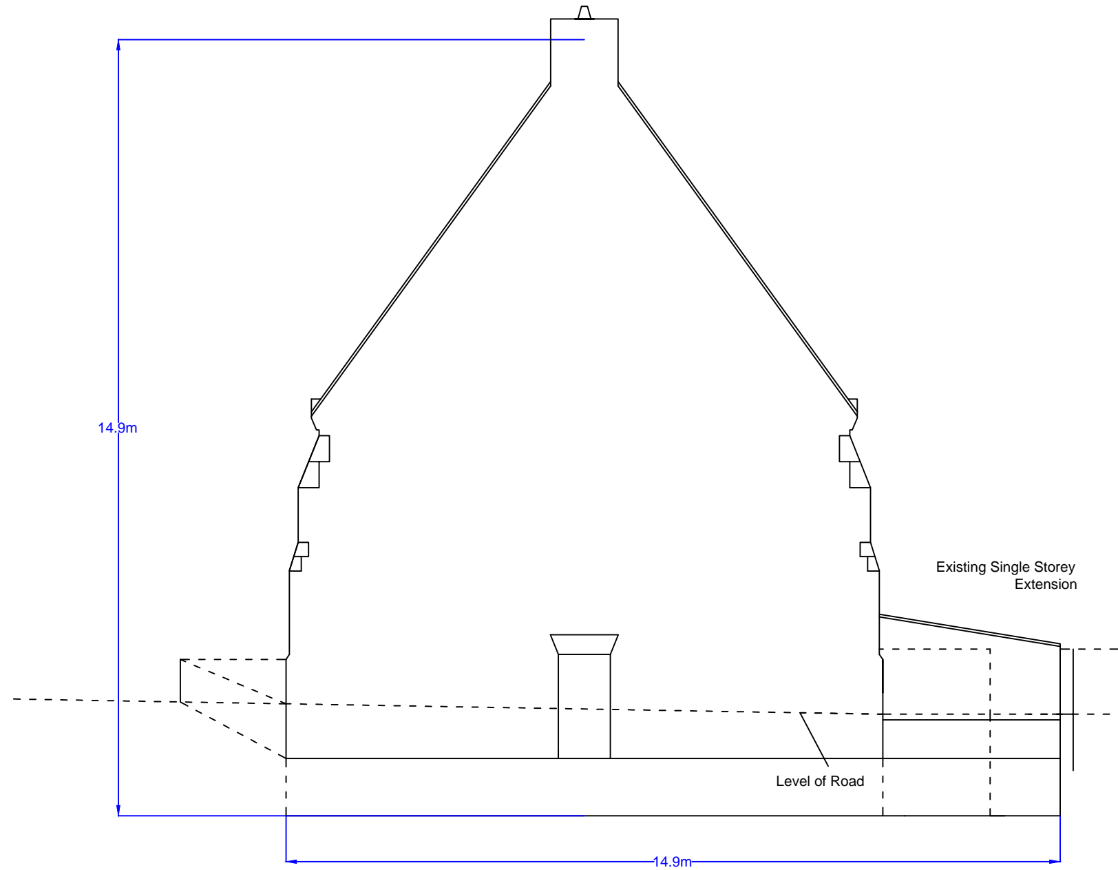
8DT9: 8 Derby Terrace South Elevation As Is Page 1 of 1, Scale 1:100 at A3
